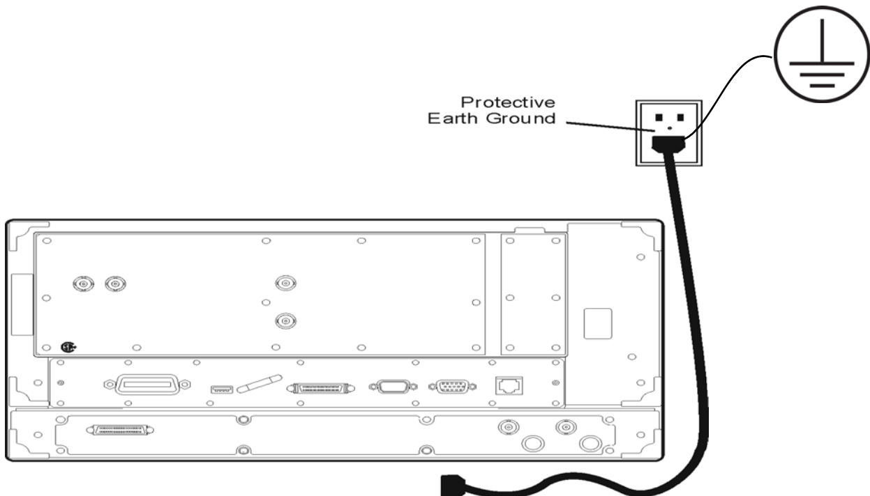
Figure 2-1 Protective Earth Ground (Non-Floating)
